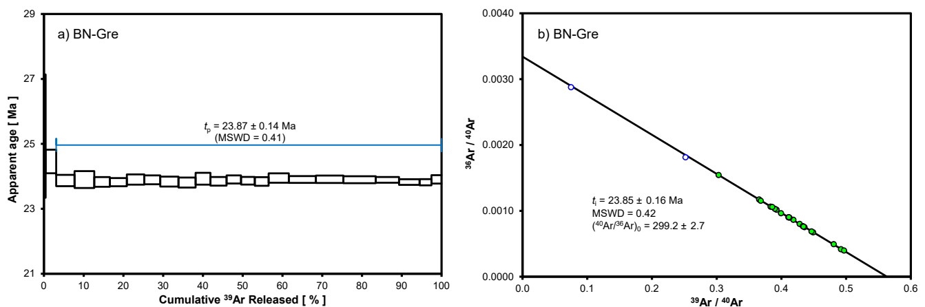
Fig. 9. (a) ^{40}\text{Ar}/^{39}\text{Ar} plateau age spectra and (b) inverse isochron of muscovite in sample BN-Gre collected at Ban Ngoc.
