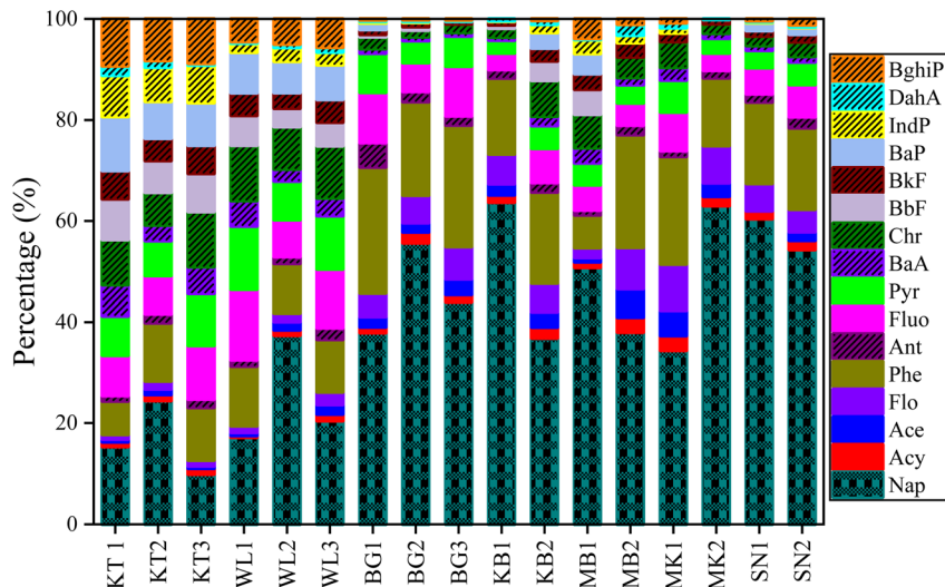
Fig. 3 The individual PAH concentrations and percentage composition in the topsoil from selected cities in Sierra Leone. KT: Kingtom, WL: Waterloo; BG: Bongonema, MB: Magburaka, MK: Makeni, KB: Kabala, and SN: Sinikoro.
