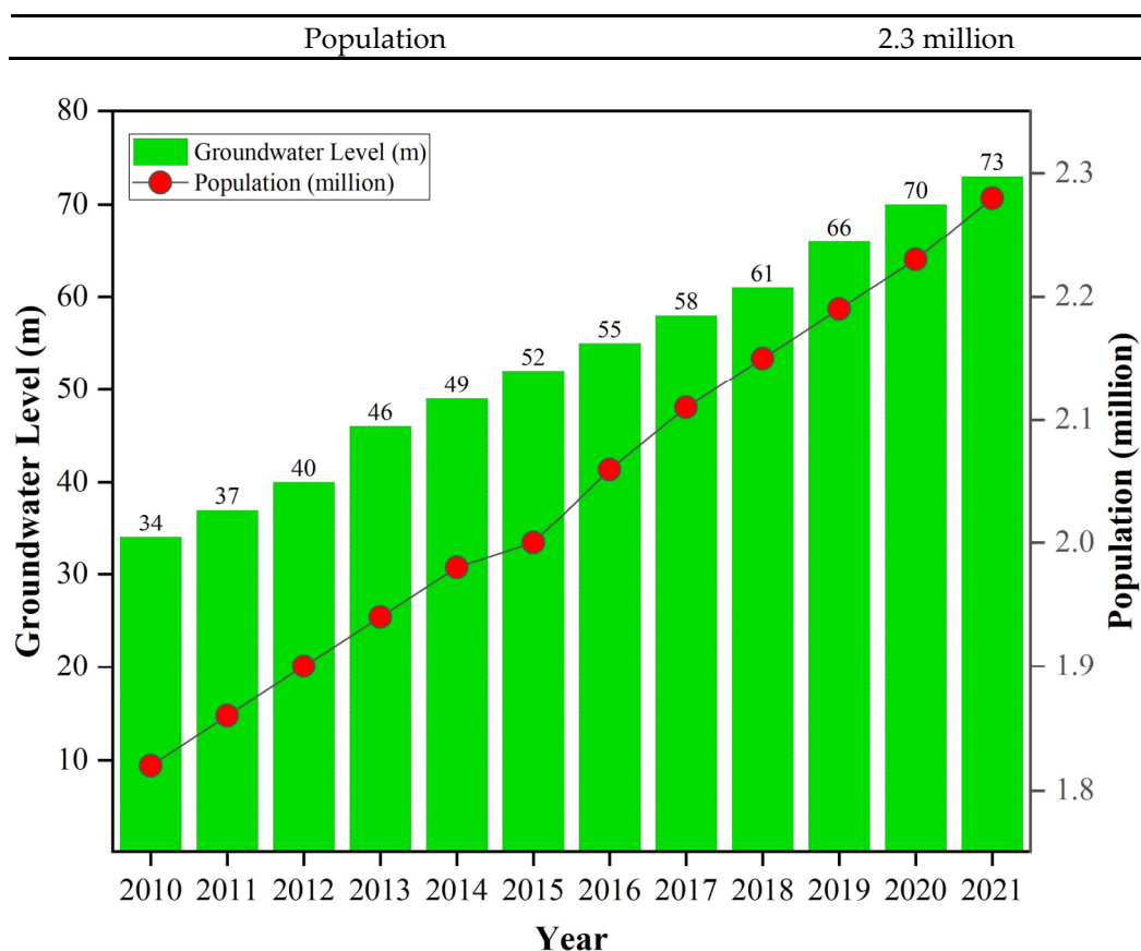
Figure 18. Changes in groundwater level with the rise in population overtime.
