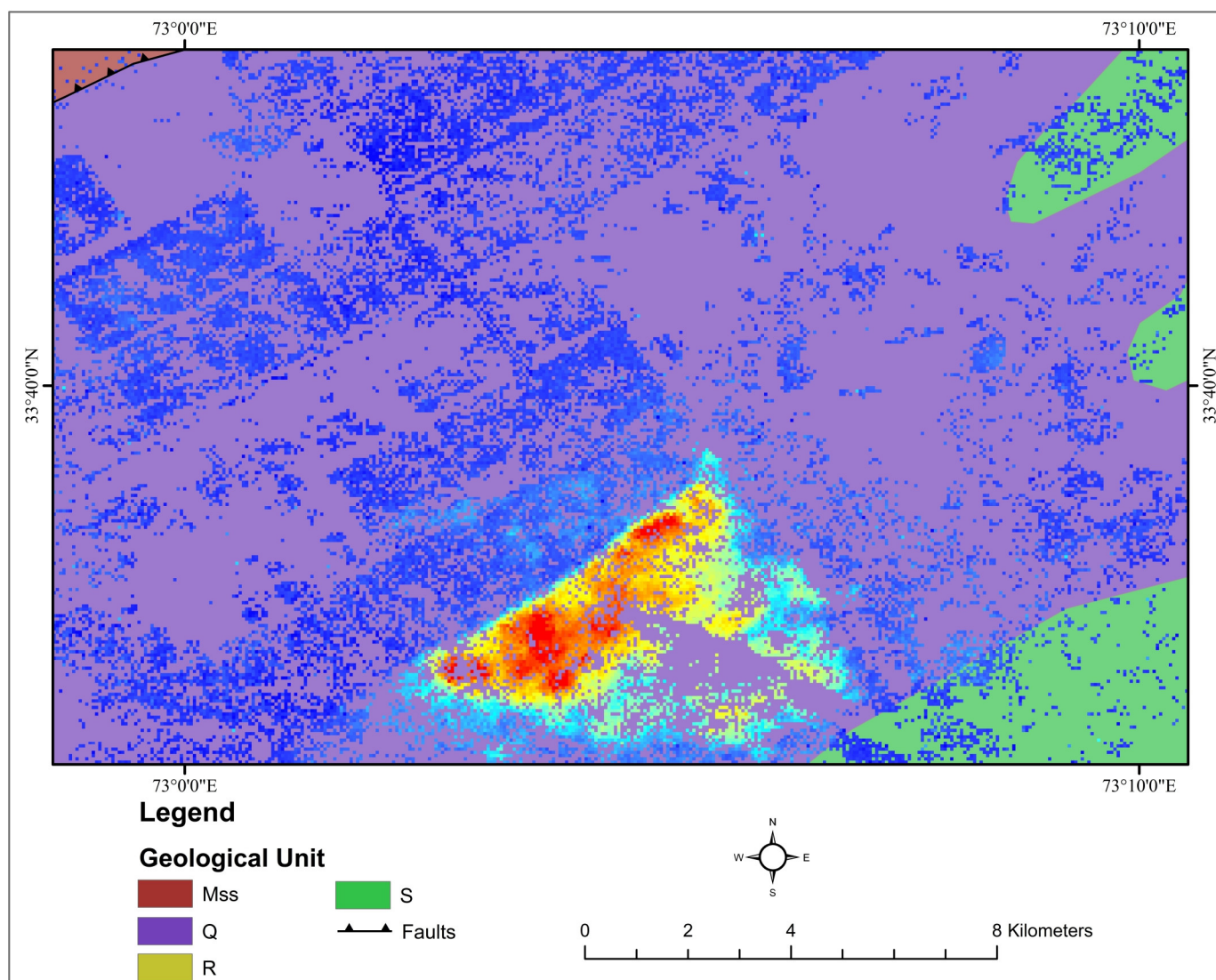
Figure 20. Subsidence along the geological map in the research area.
